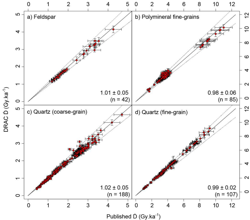
Figure 5: Comparison of dose rates ( \dot{D} ) calculated in DRAC with those previously published. Data are plotted separately for a) feldspar, b) polymineral, c) coarse-grain ( >63 \mu\text{m} ) quartz and d) fine-grain ( <63 \mu\text{m} ) quartz. 422 samples from 32 studies are compared with a mean ratio of 1.01 \pm 0.05 . If not stated in the publication, the following parameters were used to facilitate comparison: conversion factors – Adamiec and Aitken (1998), no Rb calculation from K, grain size attenuation for \dot{D}_\alpha and \dot{D}_\beta – Bell (1980) and Mejdahl (1979) respectively, etch depth – 9 \mu\text{m} , etch depth attenuation – Bell, 1979, a-value either 0.086 \pm 0.0043 , 0.035 \pm 0.001 (Rees-Jones and Tite, 1997) or 0.15 \pm 0.015 (Balescu and Lamothe, 1994) dependent on mineral and grain-size, overburden density – 2.0 \pm 0.1 \text{ g.cm}^{-3} , latitude, longitude and altitude estimated from Google Earth. The studies used for the DRAC comparison: Alappat et al., 2011, Bates et al., 2003, Breman et al., 2003, Buylaert et al., 2007 and Clark-Balzan et al., 2012, Davidovich et al., 2012, Demeter et al., 2012, Fuchs et al., 2012, Haberzettl et al., 2009, Halfen et al., 2010, Hall et al., 2010, Houben et al., 2013, Kaiser et al., 2009, Kars et al., 2012, Kels et al., 2014, Klasen et al., 2011, Kock et al., 2009, Kreutzer et al., 2012, Le Dortz et al., 2009, Lepper et al., 2013, Lomax et al., 2014, Madsen et al., 2009, Roskosch et al., 2012, Schatz et al., 2012, Schmidt et al., 2014, Schokker et al., 2005 and Stevens et al., 2011, Tamura et al., 2011, Thiel et al., 2011, Xu et al., 2010 and Yang et al., 2010.
